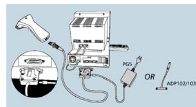
RS232
